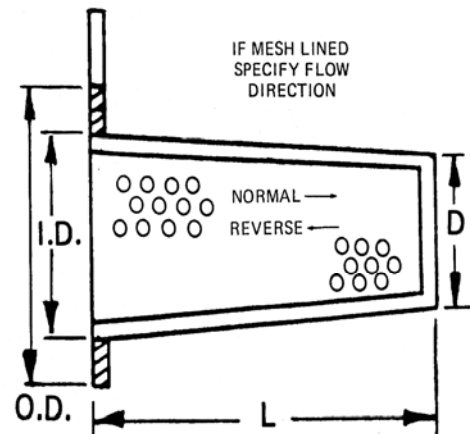
IF MESH LINED SPECIFY FLOW DIRECTION STYLE "C" CARBON STEEL STYLE "CS" STAINLESS STEEL BASKET TYPE
