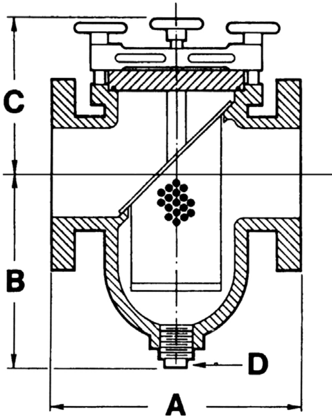
DIMENSIONS & WEIGHTS APPROXIMATE (Apply for certified drawings)
