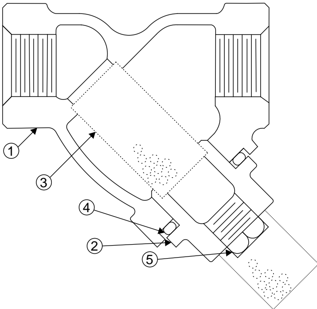
Figure 8: CAD Illustration
